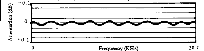
Passband Ripple Characteristics (1st stage)
