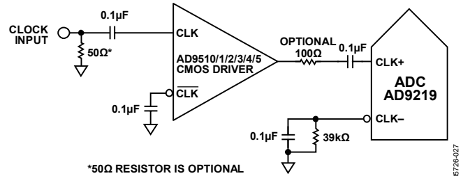
Figure 53. Single-Ended 1.8 V CMOS Sample Clock
