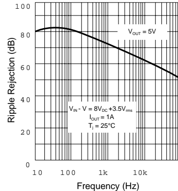
RIPPLE REJECTION
