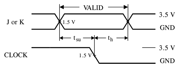
Figure 2. Switching Waveforms
