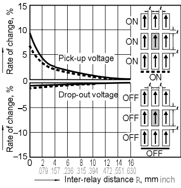
14-(3). Influence of adjacent mounting Tested sample: TXS2-4.5V, 6 pcs.
