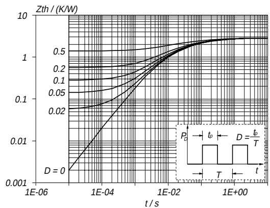
Fig.10. Transient thermal impedance. Z_{th\ j\text{-}hs} = f(t); \text{ parameter } D = t_p / T
