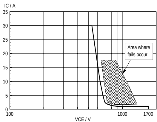
Fig.12. Reverse bias safe operating area. T_j \leq T_{j\text{max}}
