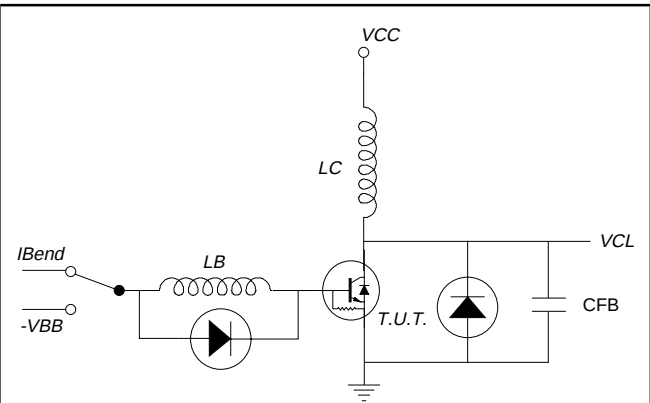
Fig.11. Test Circuit RBSOA. V_{CC} = 150\text{ V}; -V_{BB} = 1 - 4\text{ V}; L_C = 1\text{ mH}; V_{CL} = 1500\text{ V}; L_B = 0.5 - 2\text{ }\mu\text{H}; C_{FB} = 1 - 3\text{ nF}; I_{B(\text{end})} = 0.8 - 4\text{ A}
