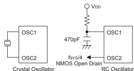
System Oscillator
