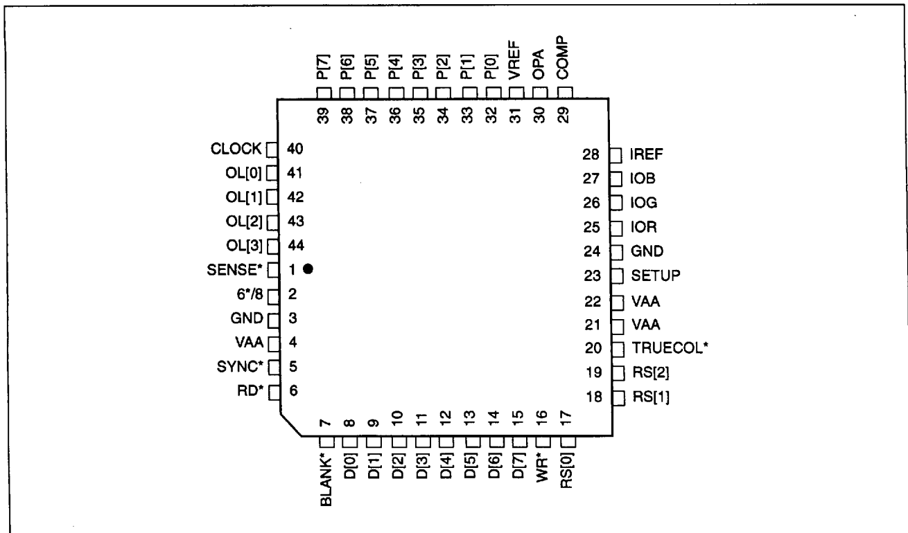
Figure 1. Pinout Diagram
