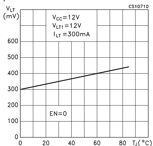
Figure 21 : Loopthrough Switch Drop Voltage vs Temperature
