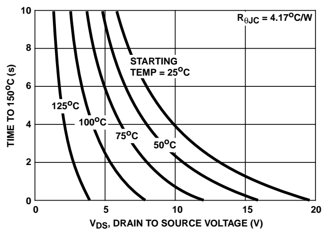
FIGURE 20. TIME TO 150°C IN CURRENT LIMITING
