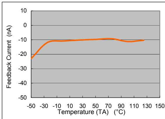
AP1518 Feedback Current v.s. Temperature (Vcc=12V, Vout=5V, Vfb=0.8V)
