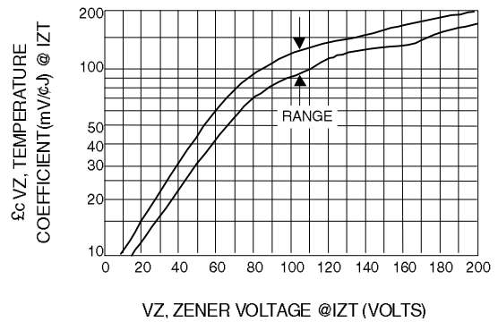
Fig. 6-UNITS 10 TO 200 VOLTS
