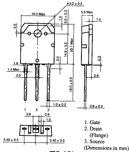
(TO-3P)
