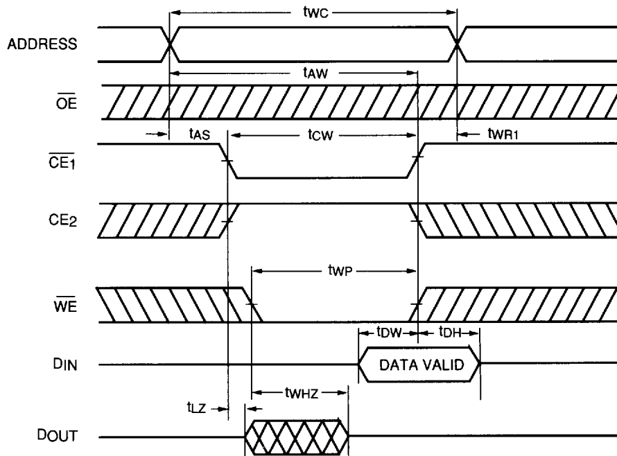
FIGURE 6. WRITE CYCLE TIMING NO. 2 ( \overline{CE1} CONTROL)
