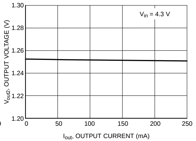
Figure 4. Output Voltage vs. Output Load Current for V out2
