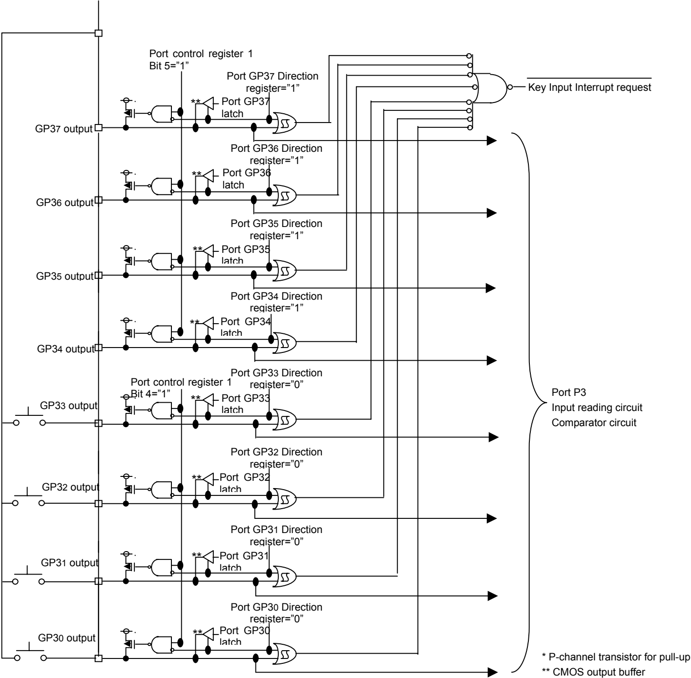
Fig.8.1 Connection Example
