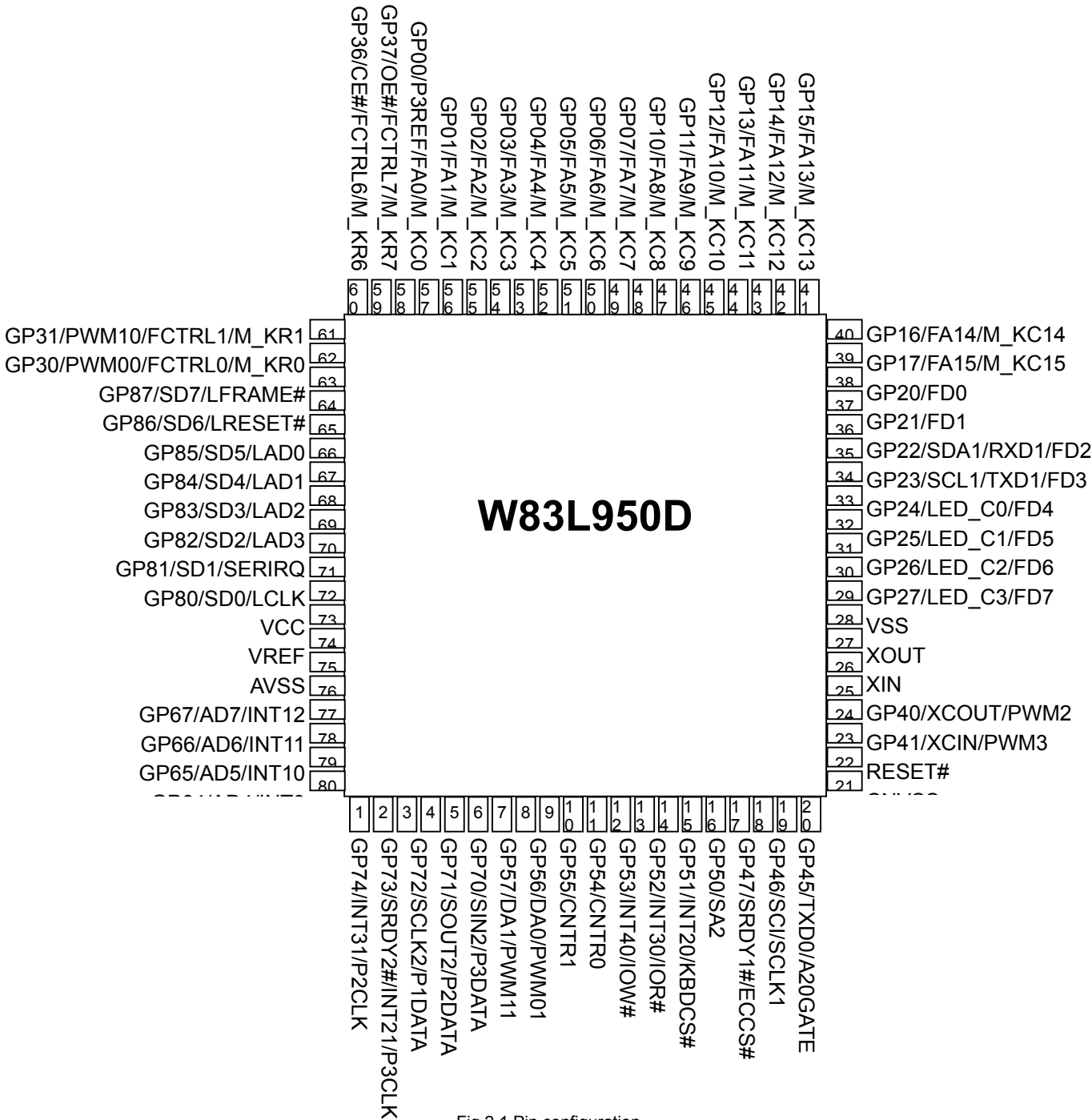
Fig 2.1 Pin configuration
