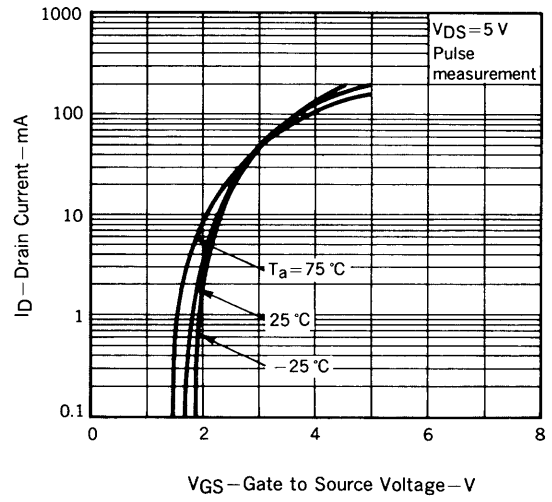
TRANSFER CHARACTERISTICS
