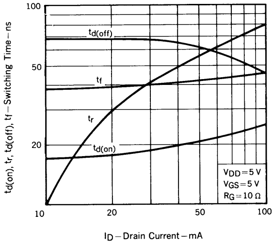
SWITCHING CHARACTERISTICS
