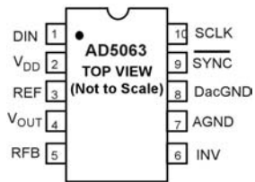
Figure 3. AD5063 10 ld uSOIC.
