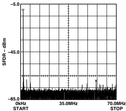
TPC 16. Single-Tone SFDR @ f_{CLOCK} = 140\text{ MHz} ( f_{OUT1} = 2\text{ MHz} )
