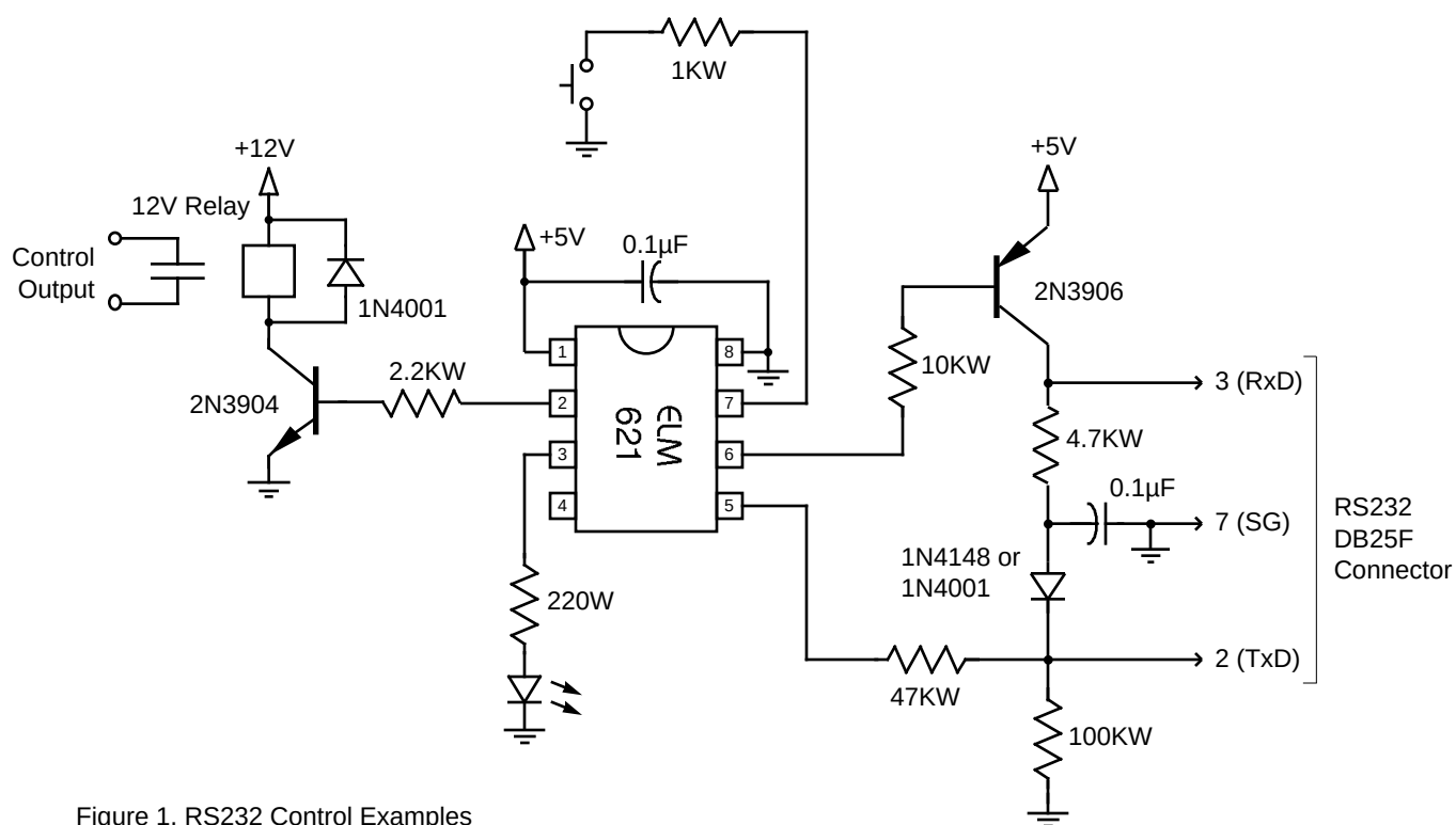
Figure 1. RS232 Control Examples
