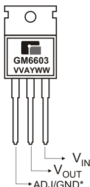
TO-220
