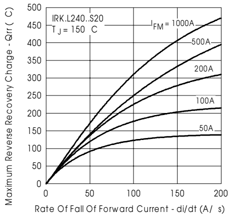
Fig. 17-ReverseRecoveryChargeCharacteristics
