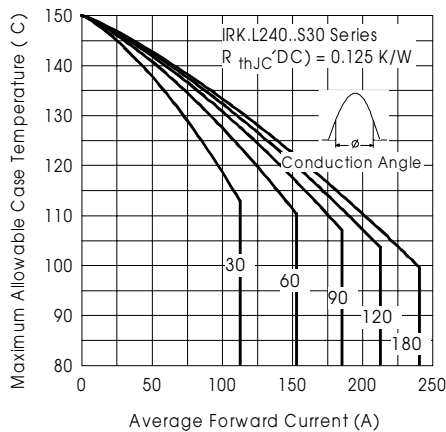
Fig. 7-Current Ratings Characteristics
