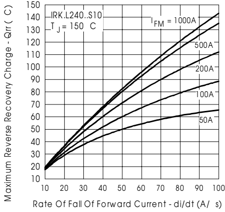
Fig. 15-ReverseRecoveryChargeCharacteristics
