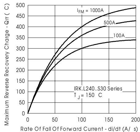
Fig. 19-ReverseRecoveryChargeCharacteristics
