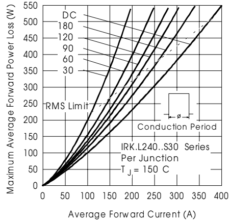
Fig.10-ForwardPowerLossCharacteristics
