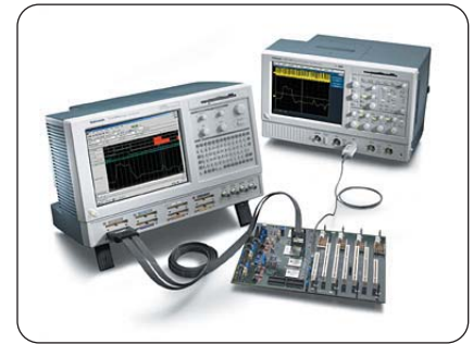
► TLA5000 Series with TDS5000 Series Oscilloscope.
