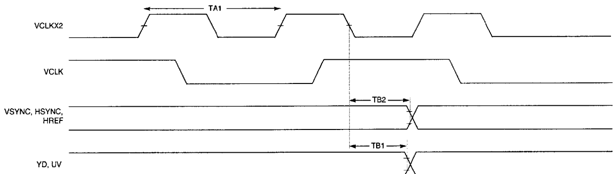
Figure 9. Digital Video Interface, Expansion
