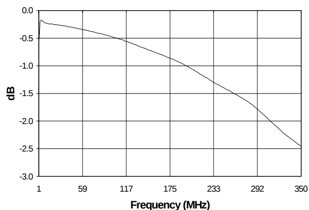
Insertion Loss
