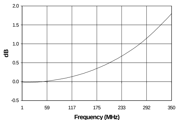
Amplitude Unbalance
