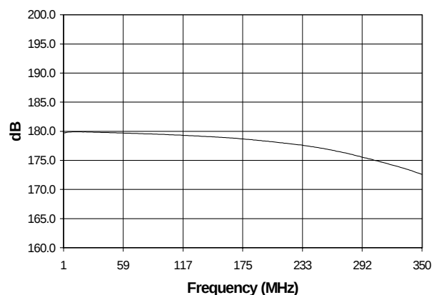
Phase Unbalance
