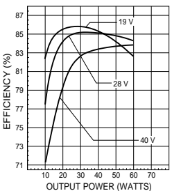
HR703-28515 EFFICIENCY VS. LINE & LOAD FIGURE 9
