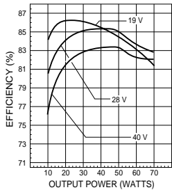
HR702-2812 EFFICIENCY VS. LINE & LOAD FIGURE 6
