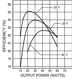
HR701-2805 EFFICIENCY VS. LINE & LOAD FIGURE 3
