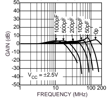
Closed-Loop Frequency Response
