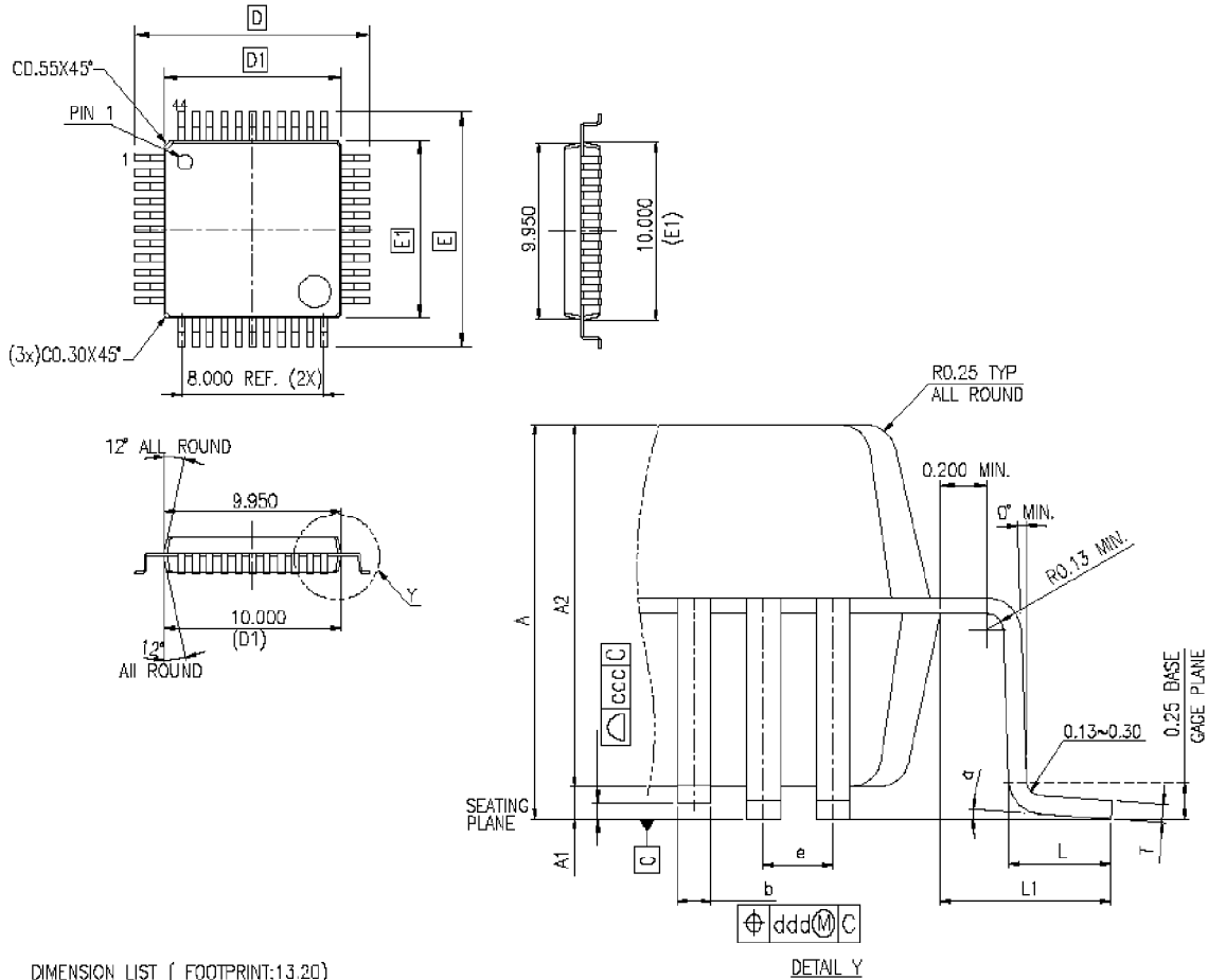
DIMENSION LIST ( FOOTPRINT:13.20)
