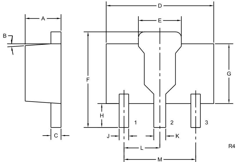
BOTTOM VIEW
