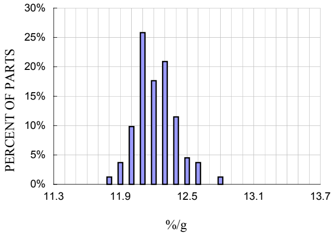
Y-axis Sensitivity Distribution at Yout, V_{DD}=3V
