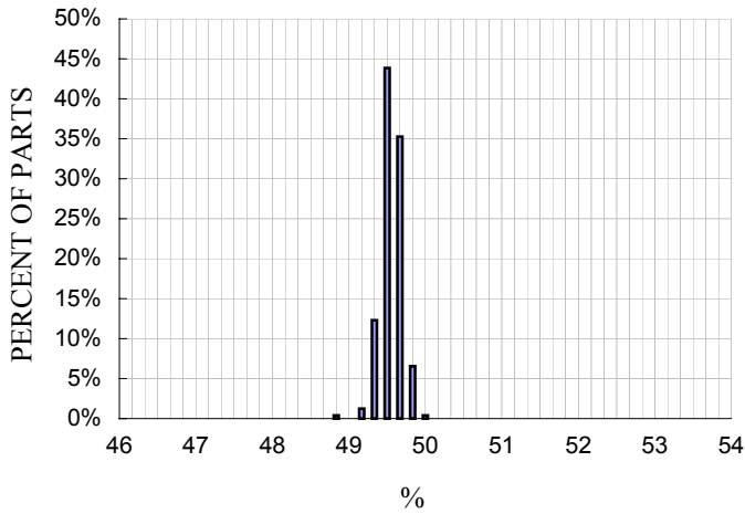
Y-axis Zero g Bias Distribution at Xout, V DD =3V
