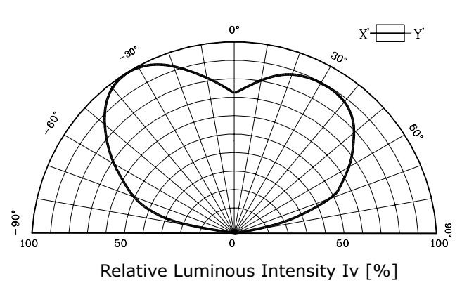
Fig. 5-2 Radiation Diagram(Y)
