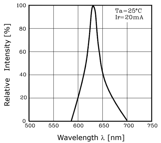
Fig.4 Spectrum Distribution
