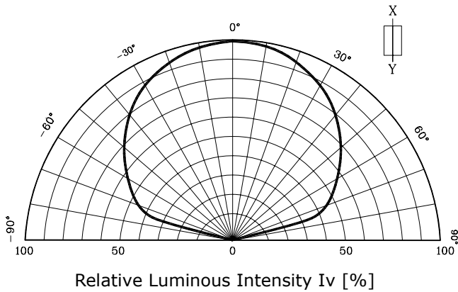
Fig. 5-1 Radiation Diagram(X)
