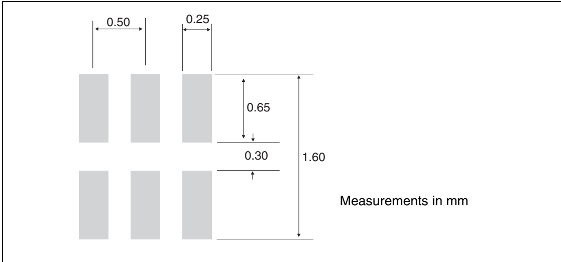
Figure 11. Footprint
