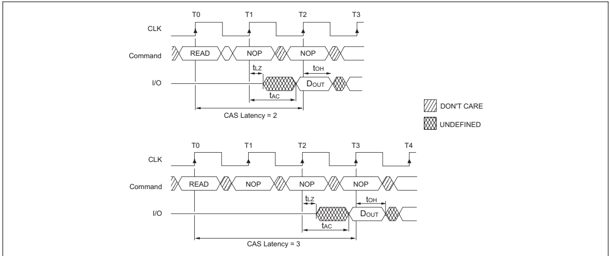
FIGURE 4 – CAS LATENCY
