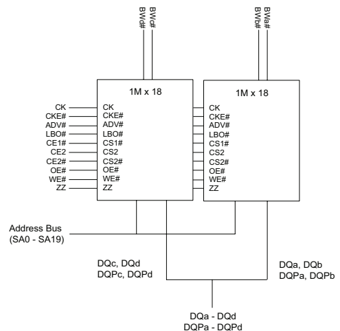
BLOCK DIAGRAM
