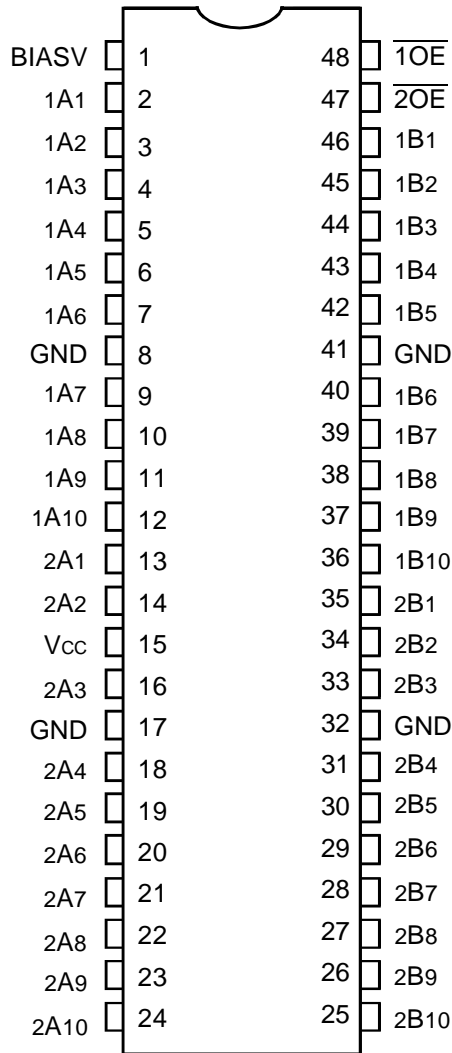
SSOP/ TSSOP/ TVSOP TOP VIEW
