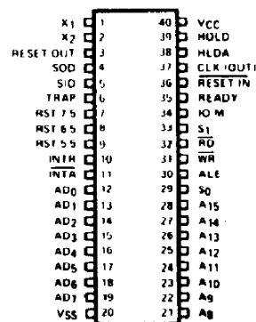
Figure 2. M8085AH Pin Configuration
