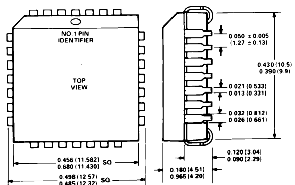
28-Terminal Plastic Ledged Chip Carrier (P-28A)
