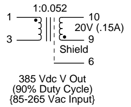
Schematic 3
