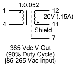
Schematic 6
