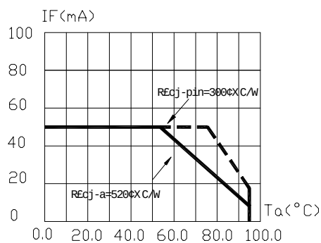
FIG.5 MAXIMUM FORWARD DC CURRENT VS AMBIENT TEMPERATURE. DERATING BASED ON T_{jmax}=105^{\circ}\text{C}
