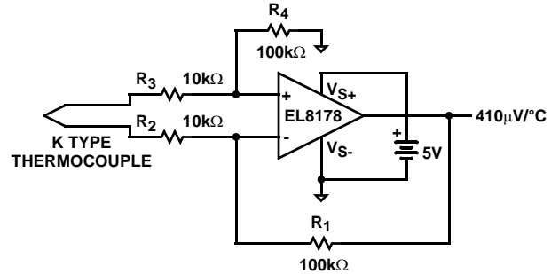
FIGURE 29. THERMOCOUPLE AMPLIFIER
