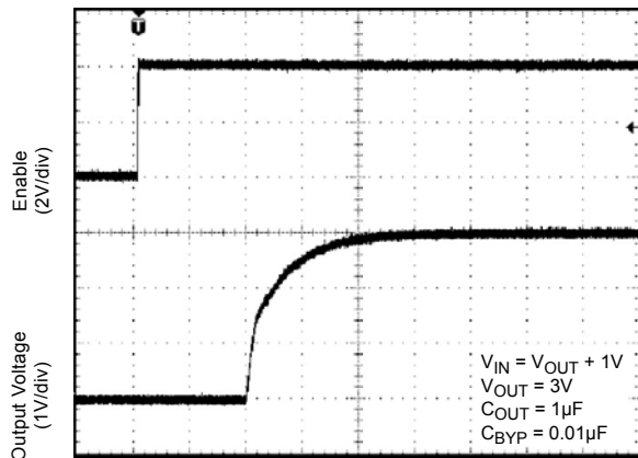
Time (10µs/div)
