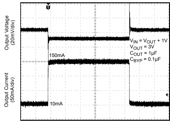
Time (40µs/div)
