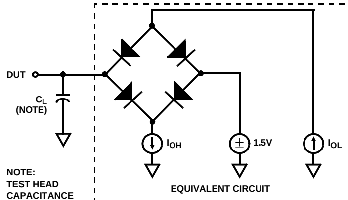
FIGURE 2. TEST CIRCUIT
