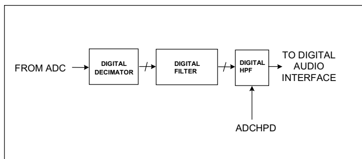
Figure 10 ADC Digital Filter
