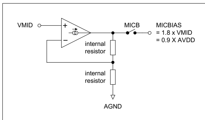
Figure 9 Microphone Bias Schematic
