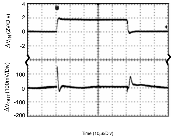
Figure 15. Line Transient (Conditions: V_{IN}=5 to 7V , I_{OUT}=1.5A , C_{OUT}=10µF )
