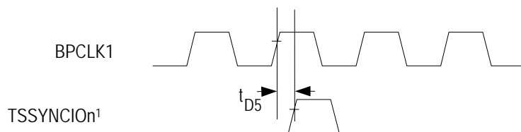
Figure 13-11. BPCLK1 Timing
