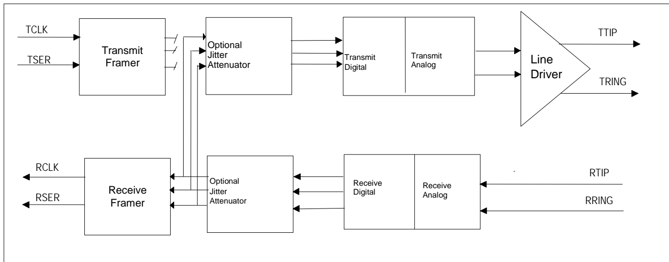
Figure 9-29. Remote Loopback 2
