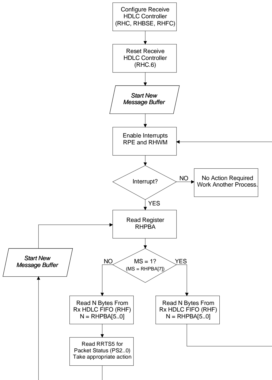
Figure 9-17. HDLC Message Receive Example
