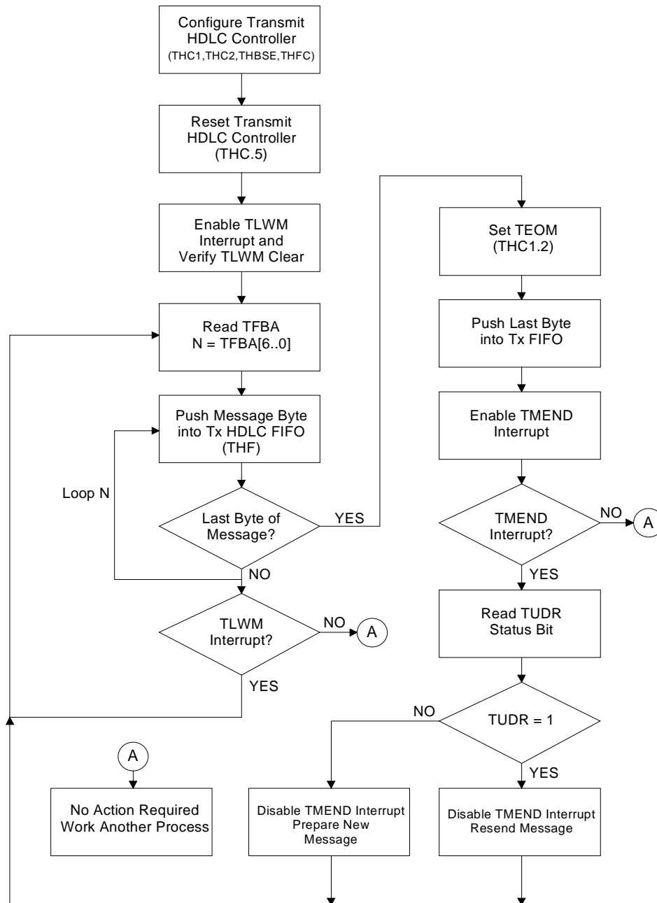
Figure 9-18. HDLC Message Transmit Example
