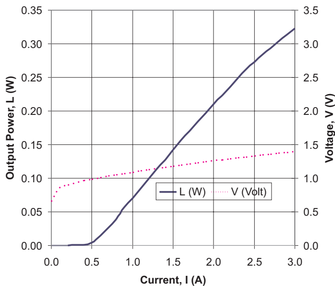
Figure 3. LIV Characteristics, CW. Light output power ( L ) is the full line. Voltage drop across the laser ( V ) is the dotted line.
