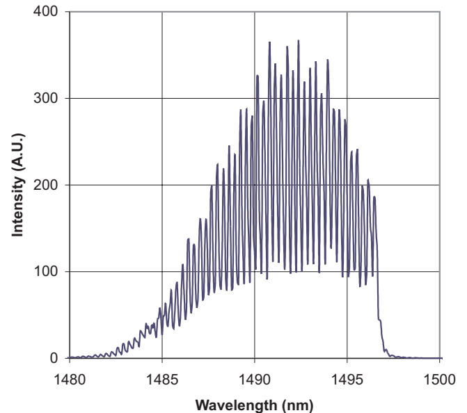
Figure 4. Spectrum from a laser with a mean wavelength of 1492 nm and a spectral bandwidth of approximately 10 nm. As an option a fine selection of the mean wavelength between 1480 and 1495 nm is possible.
