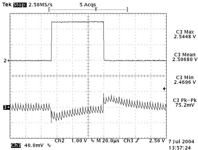
Figure 21: Typical transient response to step load change at 10A/μS from 50% to 75% and 75% to 50% of I_{o\_max} at 12Vin, 2.5V out
