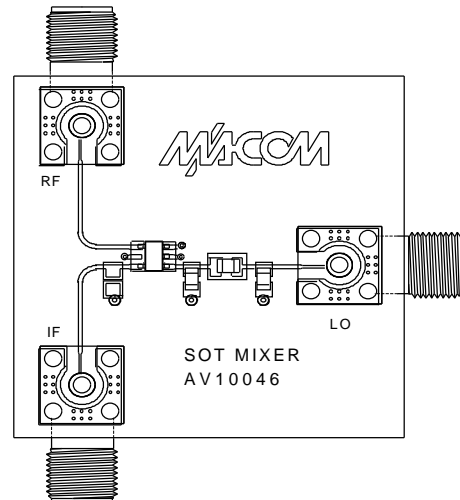
MIXER PCB
