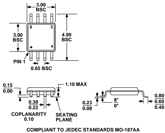
Figure 42. 8-Lead Mini Small Outline Package [MSOP] (RM-8)
