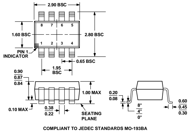
Figure 43. 8-Lead Thin Small Outline Transistor Package [TSOT] (UJ-8)
