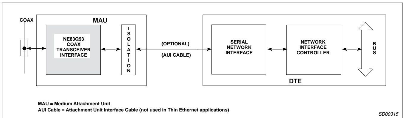
Figure 3. Interface Diagram for Ethernet/Thin Ethernet Local Area Network
