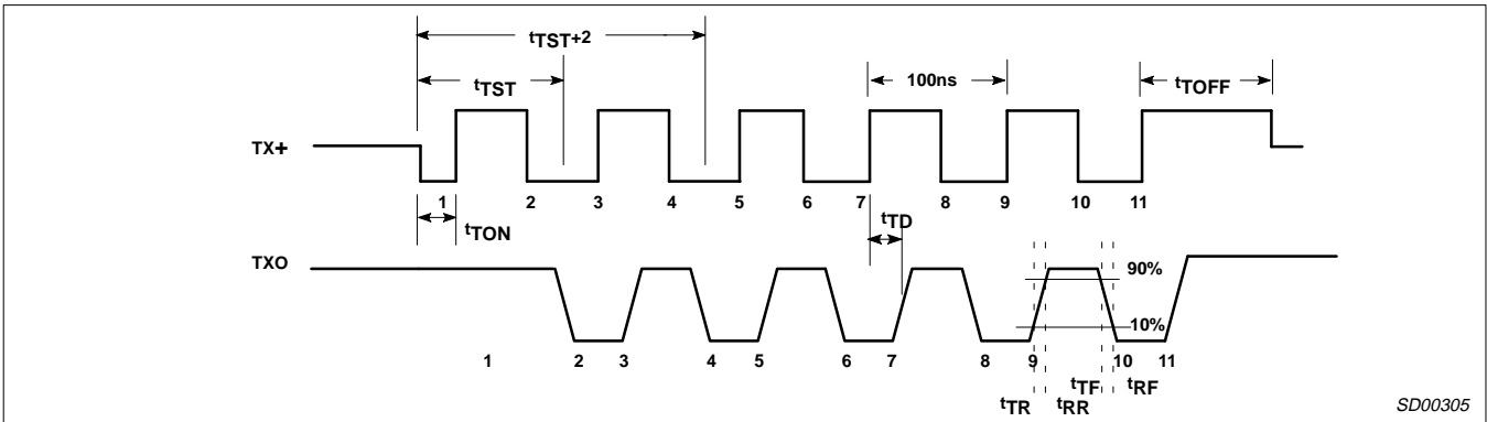
Figure 6. Transmitter Timing
